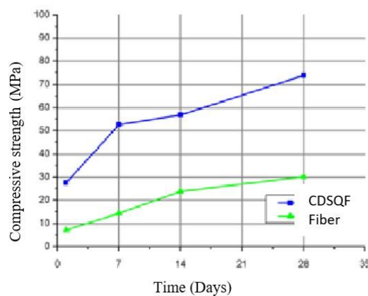
Figure 10: Mechanical compressive strengths of Mortar and UPFC
