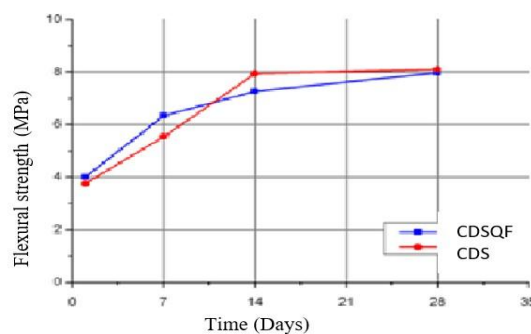
Figure 9: Kinetics of evolution of the flexural strength of the different formulations
