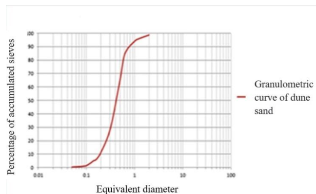
Figure 3: Granulometric curve of dune sand
