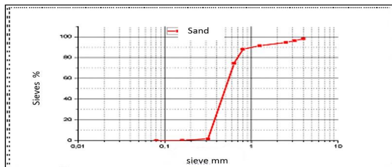
Figure 5: Particle size analysis of sand (0/3)
