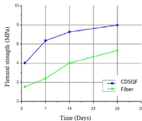
Figure 11: Mechanical resistances in bending of Mortar and UHPFRC
