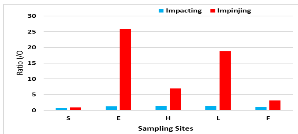
Fig4: Indoor/Outdoor Ratio for Identification of Bacterial Airborne Sources.
