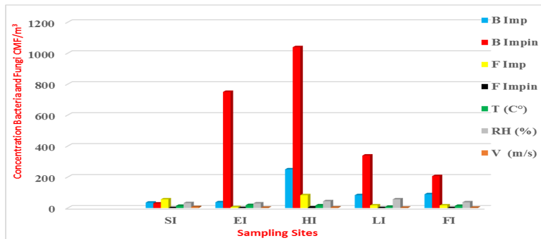
Fig2: Indoor Concentration of Bacteria and Fungi Airborne in Industrial and Urban Areas of Ouargla Region-Algeria
