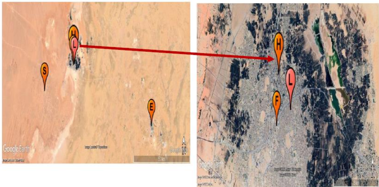
Fig.1: Sampling sites for measurement of Bioaerosol airborne in Industrial and Urban areas in Ouargla Region-Algeria
