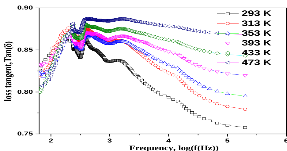
Figure 10. Loss tangent ( \tan \delta ) versus frequency (in log scale) for the cross-linking (TPGDA)/MMt-Cs + nanocomposite.
