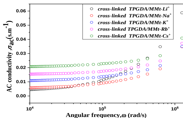
Figure 7. Ac conductivity spectra as function of angular frequency measured at 313K for the cross-linking (TPGDA)/MMt-M + nanocomposite.
