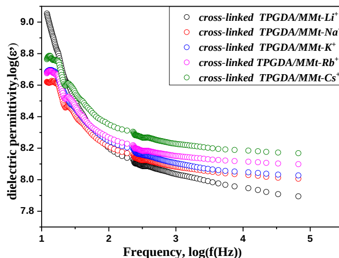
Figure 11. Real part of dielectric permittivity( \epsilon' )versus frequency (in log-log scale)at 313K for the cross-linking (TPGDA)/MMt- M^+ nanocomposite.
