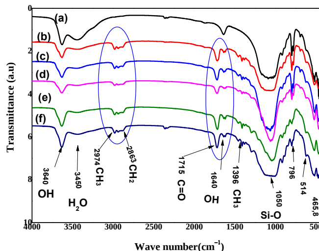
Figure 5. FTIR spectra of : (a) MMt- \text{Na}^+ , (b) cross-linking (TPGDA)/MMt- \text{Li}^+ nanocomposite, (c) cross-linking (TPGDA)/MMt- \text{Na}^+ nanocomposite, (d) cross-linking (TPGDA)/MMt- \text{K}^+ nanocomposite, (e) cross-linking (TPGDA)/MMt- \text{Rb}^+ nanocomposite and (f) cross-linking (TPGDA)/MMt- \text{Cs}^+ nanocomposite.
