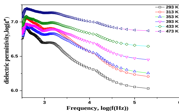
Figure 9. Imaginary part of dielectric permittivity ( \epsilon'' ) versus frequency (in log-log scale) at different treatment temperatures in the case of the cross-linking (TPGDA)/MMt- \text{Cs}^+ nanocomposite.
