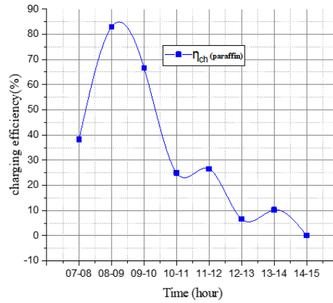
Figure.14 The variation of charging efficiency with time in the presence of the storage material.
