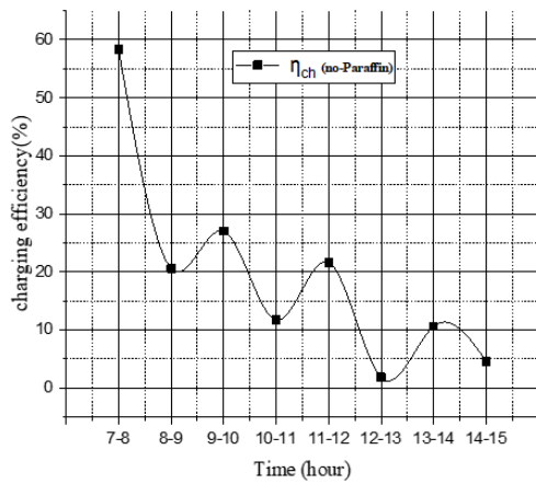
Figure.13 The variation of charging efficiency with time in the absence of the storage material(presence of air).
