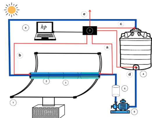
1. Parabolic Trough Collector 2. Copper absorber tube, 3. Glass envelope, 4. Water storage tank, 5. Pump, 6. flow meter device, 7. Arduino 8. computer, a,b,c,d,e Thermocouples.
