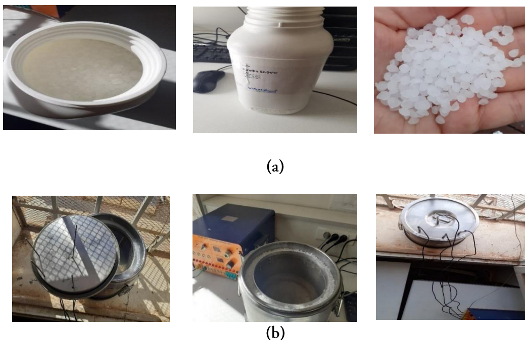
Figure. 1 (a) Paraffin wax used, (b) Thermal storage tank.
